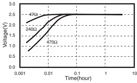
Charge Characteristics (Charge Voltage 2.5V)
