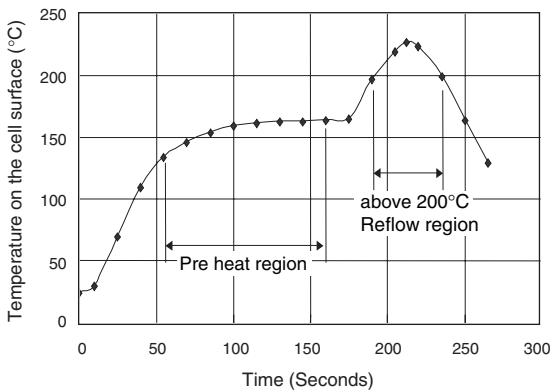
Reflow Soldering Temperature Profile Example
