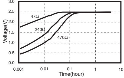
Charge Characteristics (Charge Voltage 2.5V)
