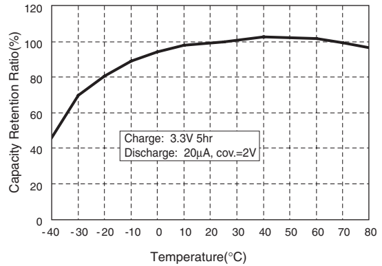
Temperature Characteristics
