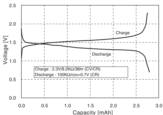
Charge/discharge characteristics
