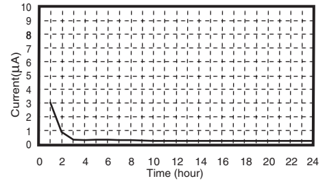
Leak Current Characteristics (Charging at 2.5V)
