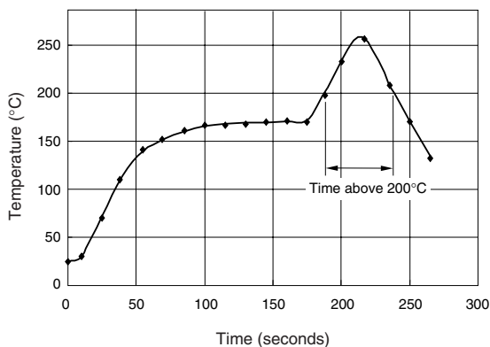
Reflow soldering profile (for reference only)
