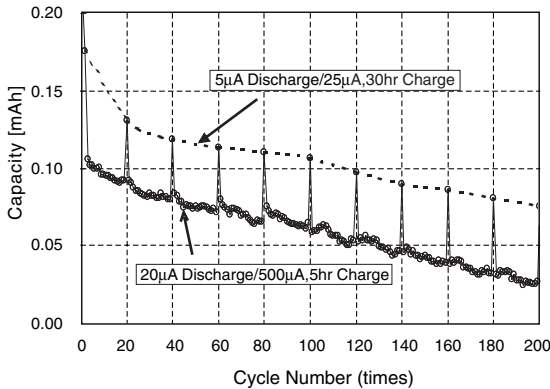
Charge-Discharge Cycle Characteristics (100% D.O.D)
