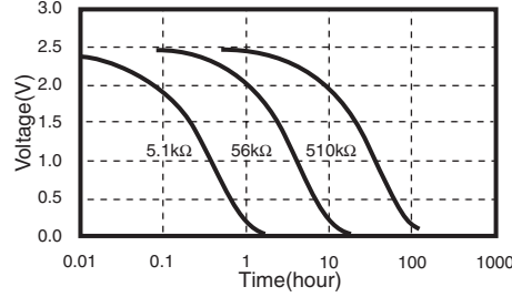
Discharge Characteristics (constant resistance)
